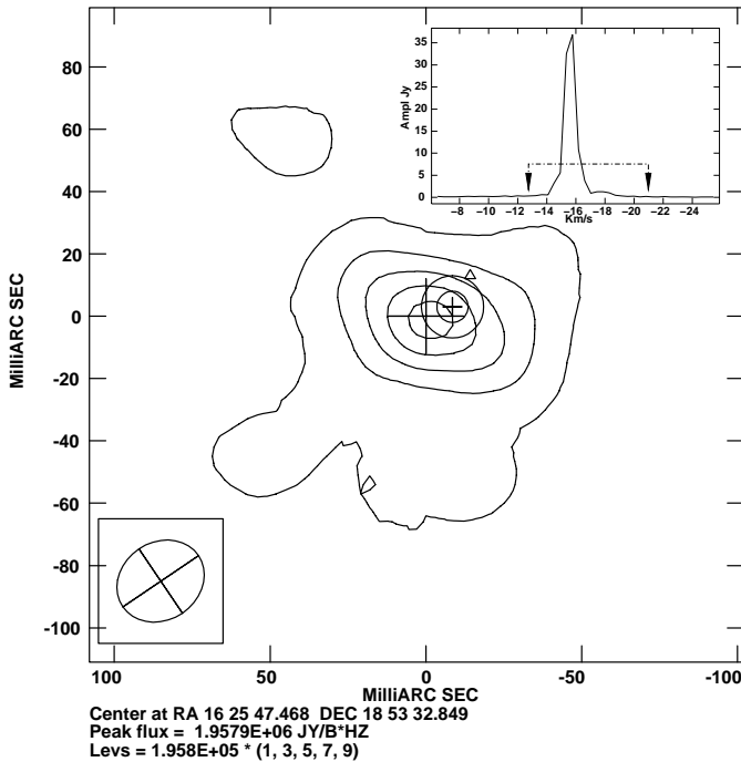
Fig. 1. The location of the U Her H 2 O masers with respect to the stellar positions determined from the Hipparcos observations, as determined from phase referencing to J1628+214. The star is denoted by two circles indicating the star itself and the stellar radio photo-sphere. The large cross indicates the position of the H 2 O maser, the error bars are due to the positional fitting. The errors on the stellar position (small cross) are due to the link to the radio-reference frame and due to the errors in the proper motion used to transpose the optical position. The triangle denotes the stellar position when using the phase referencing results on the J1619+2247 reference source. The inlay is the averaged cross-power spectrum of the H 2 O maser emission. The masers were mapped over the velocity range indicated in the spectrum.
