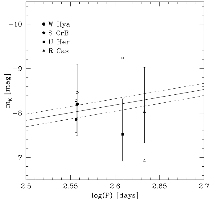
Fig. 12. Period vs. K_0 luminosity for the observed stars. The solid symbols and the error bars are determined using the distances obtained in this paper. The open symbols are the values using the Hipparcos distances. The solid line is the P – L relation determined by Whitelock & Feast (2000) on the oxygen rich Mira stars observed with Hipparcos, the dashed lines are the spread in the relation due to the error in the P – L relation zero-point.
