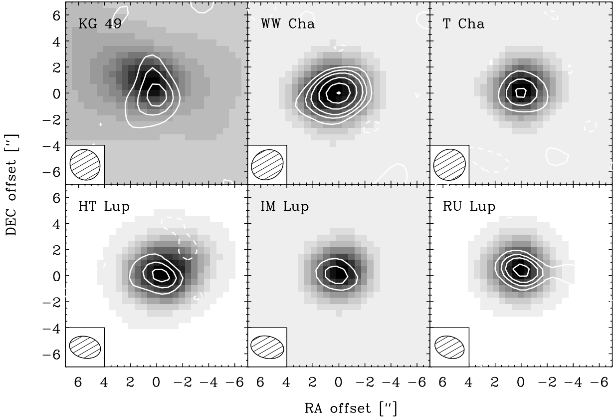
Fig. 1. ATCA images of the \lambda = 3.3 -mm continuum emission (contours), overplotted on 2MASS K -band ( 2.1 \mu\text{m} ) images (grayscale). Contour levels are drawn at 2, 4, 6, 10, 15, and 20 times the noise level; negative contours are dashed. The positional offsets are with respect to the fitted coordinates (see Table 3).
