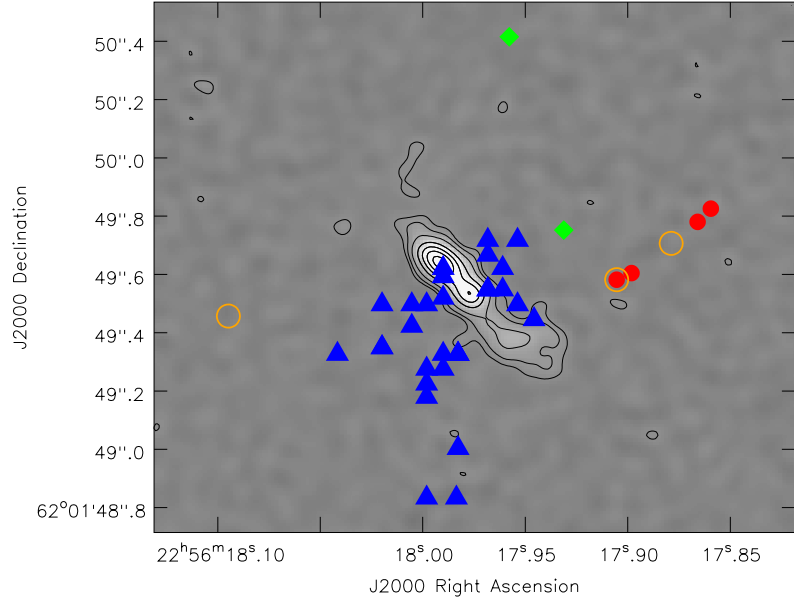
Figure 2. The source HW2 in star forming region Cep A. The background represents the 22 GHz continuum and the triangles are the locations of H_2O masers. The filled circles indicate the 6.7 GHz methanol masers positions, the open circles the 12 GHz methanol masers and the diamonds the methanol maser emission at 107 GHz. (van Langevelde & Philips, in preperation).
