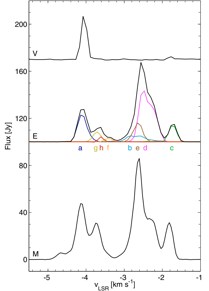
Fig. 2. Bottom: (M) Merlin 6.7 GHz maser spectrum scaled down by a factor of 5 ( Vlemmings et al. 2010 ). Middle: (E) Our 6.7 GHz total maser spectrum (black line) and individual spectra of maser clumps, from East (a) to West (h) as measured by the EVN. Top: (V) A representative 12.2 GHz maser spectra measured with the VLBA scaled up by factor of 5.
