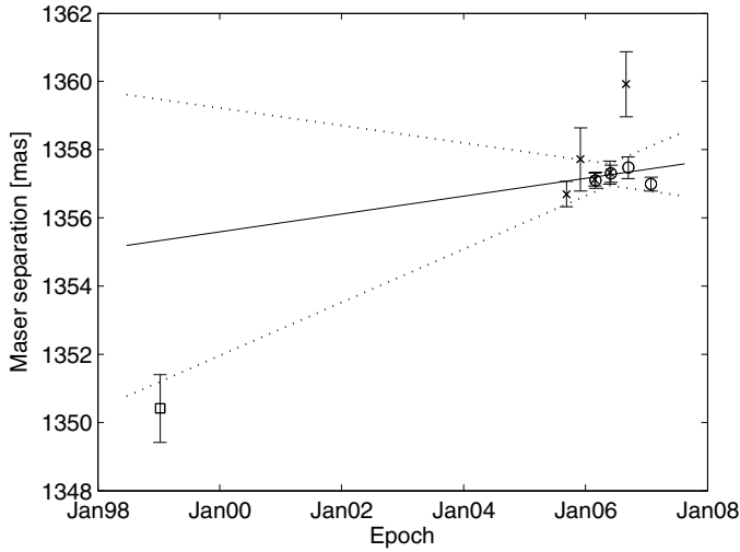
Fig. 3. Separation of the 12.2 GHz maser clumps in mas. Our four epochs are marked as circles, also shown are previous measurements by Mos01 (square) and Mos09 (crosses). The solid line indicates our best fit and the dotted lines the errors of the fit.
