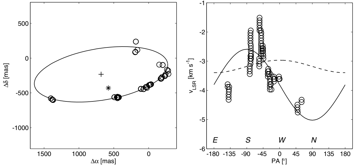
Fig. 4. Fit of the ring model: left panel shows the maser positions in circles and the fitted ellipse, with the + sign designating the centre of the ellipse. The star indicates the position of the 7 mm continuum object identified by Curiel et al. (2006). Right panel shows the measured velocities (circles) as a function of the position angle (PA) in our ring model. The solid line shows the fit to a radial velocity model and the dashed line shows the result of a Keplerian velocity model.
