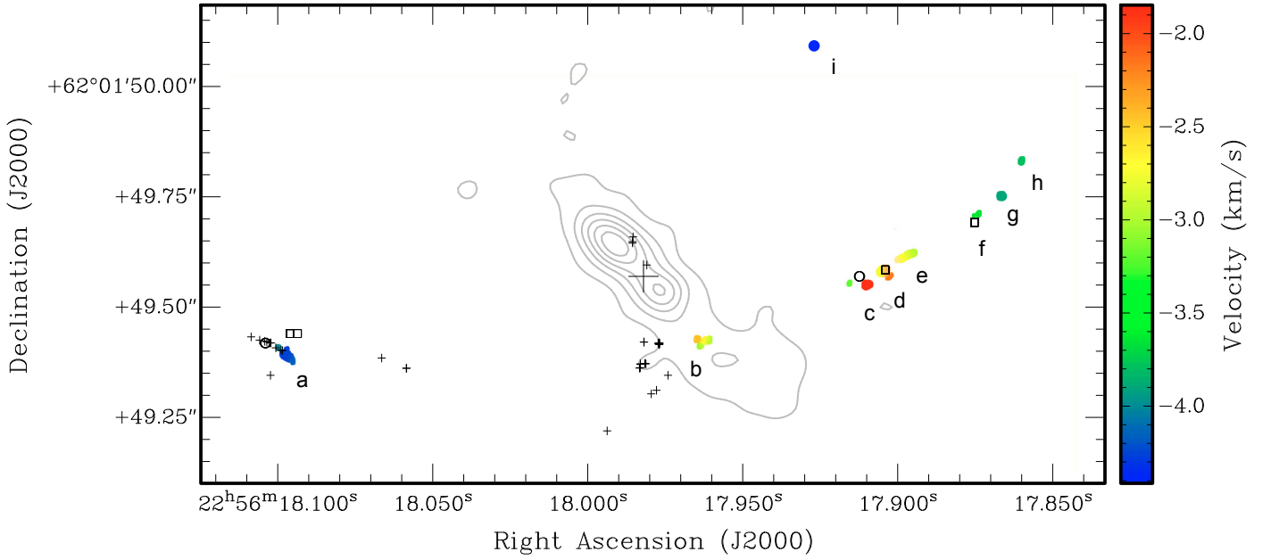
Fig. 1. The velocity field of the 6.7 GHz methanol masers as obtained from a first moment map of the bright methanol emission (colour) with labels a–i overlaid on K band continuum (contours) (Torrelles et al. 1998). The filled circle indicating the weak feature i has been added to the moment map manually based on the results of detailed fitting of each channel. Also shown are the 12.2 GHz methanol masers (circles) in this paper and (boxes) Min01, and 22 GHz water masers (small pluses) (Vlemmings et al. 2006). The position of the protostar is indicated by the large plus sign (Curiel et al. 2006).
