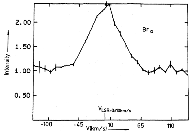
Fig. 3. Br \alpha line profile of IRAS 17516
