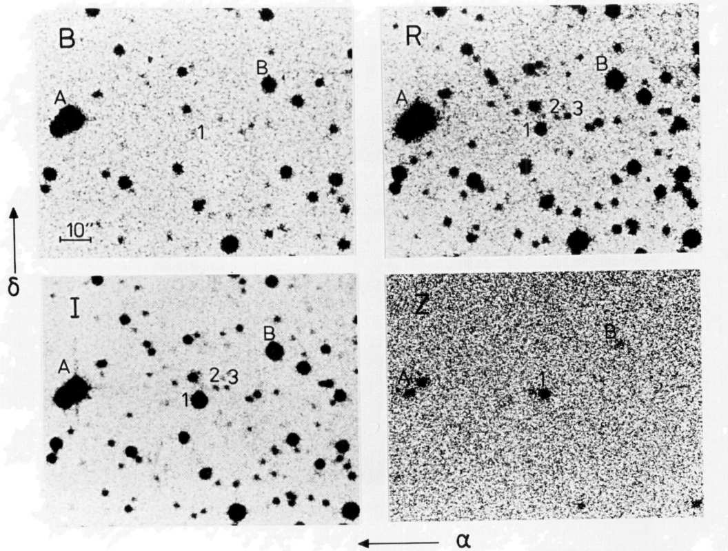
Fig. 4. Pictures taken from the ESO B plate, the ESO R plate, the SRC I plate and the UKSTU Z plate
