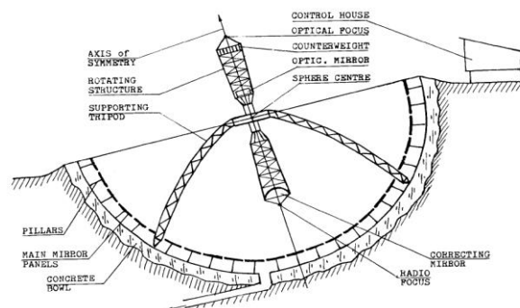
Figure 1. Arrangement of Radio-Optical Telescope ROT-54/2.6.
